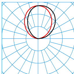
Sanesca W2 LED2600-840 03 (room light) TX046355 ■ C0 - C180 ■ C90 - C270 DIN 5040: E03 UTE: 0,00 J + 1,00 T CEN Flux Code: 0 0 0 0 100 51 81 96 100
