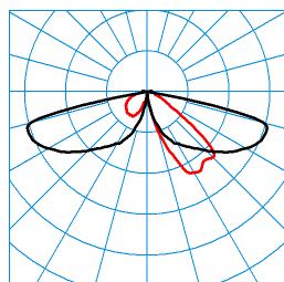
CS 19 100-AB2L/3200-740 4G1S ETDD (CLO initial value) TX300017 ■ C0 - C180 ■ C90 - C270 DIN 5040: A20 UTE: 1,00 l CEN Flux Code: 27 65 96 100 100 0 0 0 0
