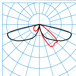
CS 19 100-AB2L/3200-740 4G1S ETDD (CLO end value) TX300016 ■ C0 - C180 ■ C90 - C270 DIN 5040: A20 UTE: 1,00 l CEN Flux Code: 27 65 96 100 100 0 0 0 0
