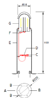
VERSION ANCRAGE STANDARD
