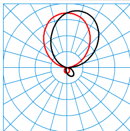
Sanesca W3-S1/R LED5000-830 03 TX050878 DIN 5040: D33 UTE: 0,12 E + 0,88 T CEN Flux Code: 43 75 93 12 100 50 80 96 88
