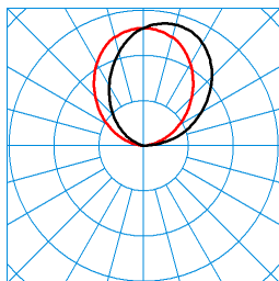
Sanesca W3-S1/R LED5000-830 03 (night light) TX055778 DIN 5040: E03 UTE: 0,00 J + 1,00 T CEN Flux Code: 0 0 0 0 100 50 81 96 100
