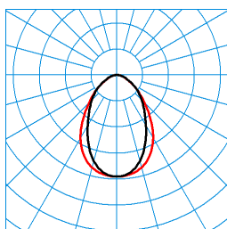
ArimoFit G2 Act D DW19 42-8 ETDD8 01/01 (ACTDSU) TX377196 ■ C0 - C180 ■ C90 - C270 UGR I = 18,1 UGR q = 18,1 DIN 5040: A50 UTE: 1,00 C CEN Flux Code: 62 88 98 100 100 0 0 0 0
