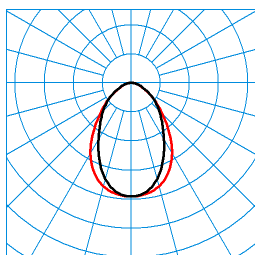
ArimoFit G2 Act D DW19 42-8 ETDD8 01/01 (ACTDCW) TX377339 ■ C0 - C180 ■ C90 - C270 UGR I = 18,1 UGR q = 18,1 DIN 5040: A50 UTE: 1,00 C CEN Flux Code: 62 88 98 100 100 0 0 0 0
