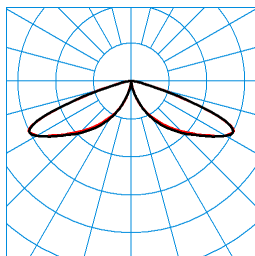
LTX KT-RB6L-LRA/15/18/26-740 4G1 (2600 lm) TX084069 ■ C0 - C180 ■ C90 - C270 DIN 5040: A20 UTE: 1,00 J CEN Flux Code: 15 51 96 100 100 0 0 0 0
