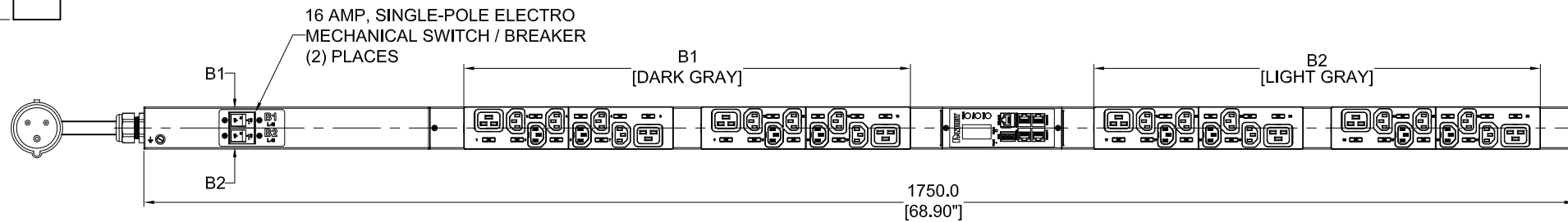
FRONT VIEW
