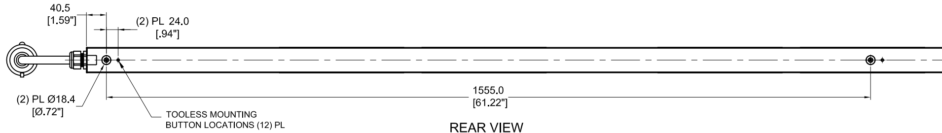
REAR VIEW
