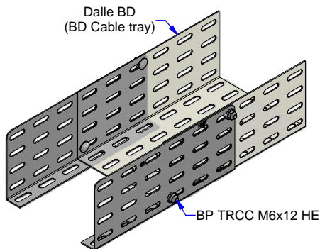
BP TRCC M6x12 HE
