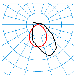
TugraHE 21 PAW 75-125/16ML-830 ET PC 23 (STAG15) TX425182
