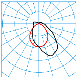
TugraHE 21 PAW 75-125/16ML-830 ET PC 23 (STAG12) TX425266
