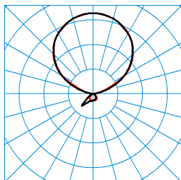
LuceoS Act S-U SMC PAW-IL 300 ETDI 01 (ACTSU) (LEO2) TX369873 C0 - C180 C90 - C270 DIN 5040: E03 UTE: 0,08 D + 0,91 T CEN Flux Code: 53 86 96 8 100 49 82 98 92
