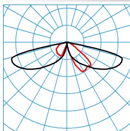
CS 19 100-AB2L/2200-730 2G1S ETDD (CLO end value) TX299970 DIN 5040: A20 UTE: 1,00 l CEN Flux Code: 26 63 96 100 100 ■ C0 - C180 ■ C90 - C270
