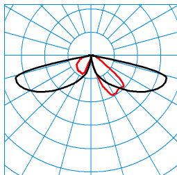
CS 19 100-AB2L/2200-730 2G1S ETDD (CLO initial value) TX299971 DIN 5040: A20 UTE: 1,00 l CEN Flux Code: 26 63 96 100 100 ■ C0 - C180 ■ C90 - C270
