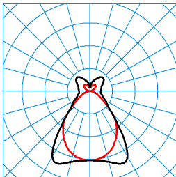
E-Line 7651 HE PMW19 40-830ET L150 01 TX375120 ■ C0 - C180 ■ C90 - C270 DIN 5040: B42 UTE: 0,72 D + 0,28 T CEN Flux Code: 60 83 93 72 100 26 59 82 28
