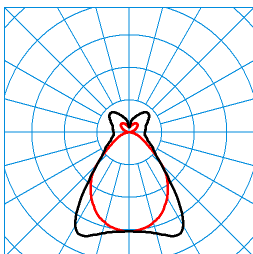
E-Line 7651 HE PMW19 40-830ETDD L150 01 TX375025 ■ C0 - C180 ■ C90 - C270 DIN 5040: B42 UTE: 0,72 D + 0,28 T CEN Flux Code: 60 83 93 72 100 26 59 82 28
