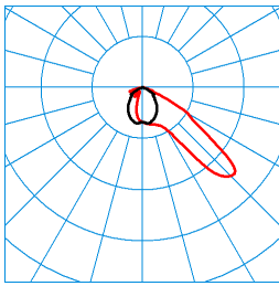
Jovie 50I-AM2L/3200-740 4G1 ETDD (CLO initial value) TX300562 ■ CO - C180 ■ C90 - C270 DIN 5040: A40 UTE: 1,00 F CEN Flux Code: 47 91 100 100 100
