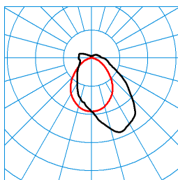
TugraHE 9 PAW 17-54/16ML-830 ET PC 23 (STAG14) TX425209 C0 - C180 C90 - C270 DIN 5040: B40 UTE: 0,86 E + 0,14 T CEN Flux Code: 48 77 92 86 100 13 32 64 14
