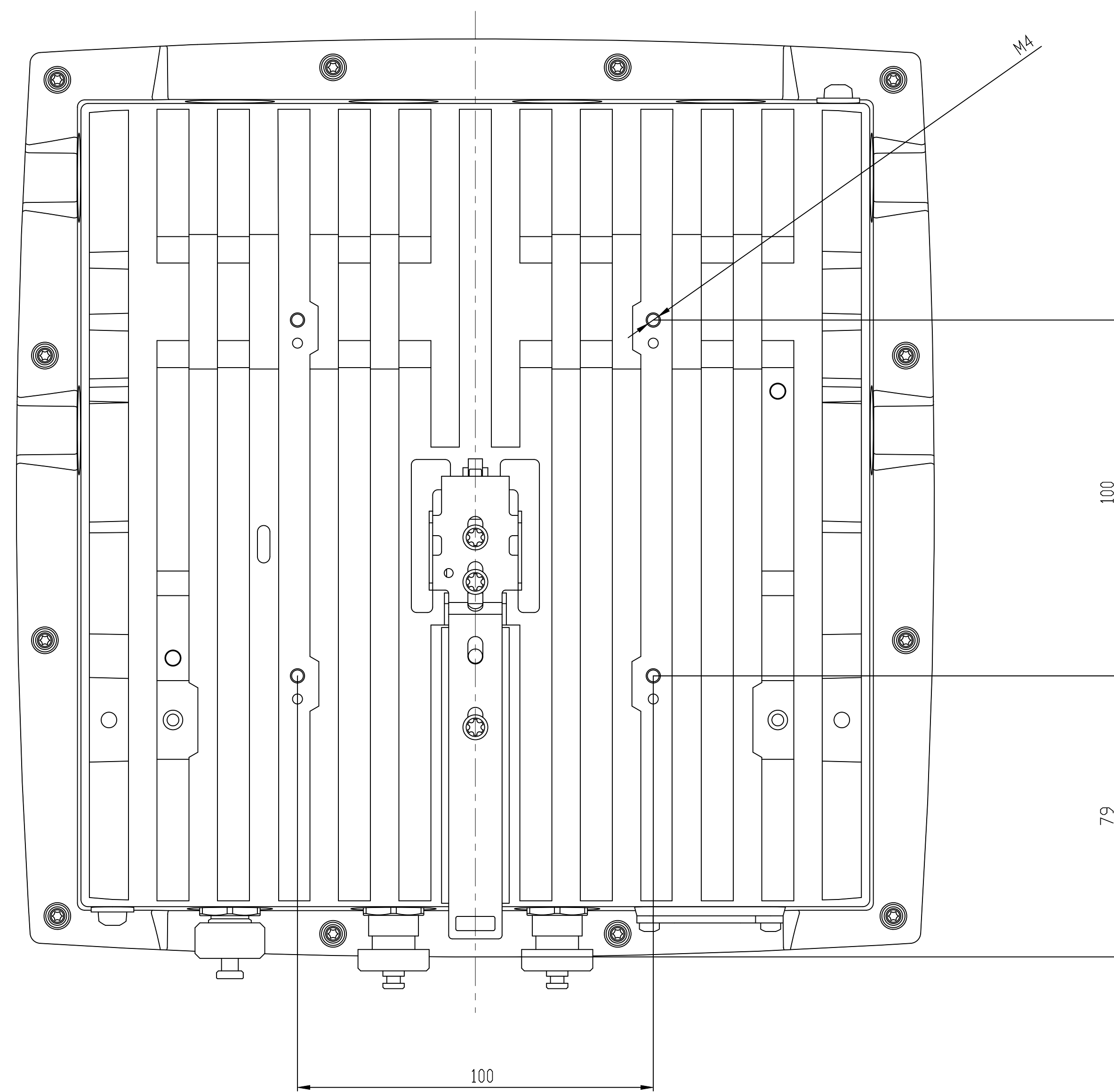
Drilling
