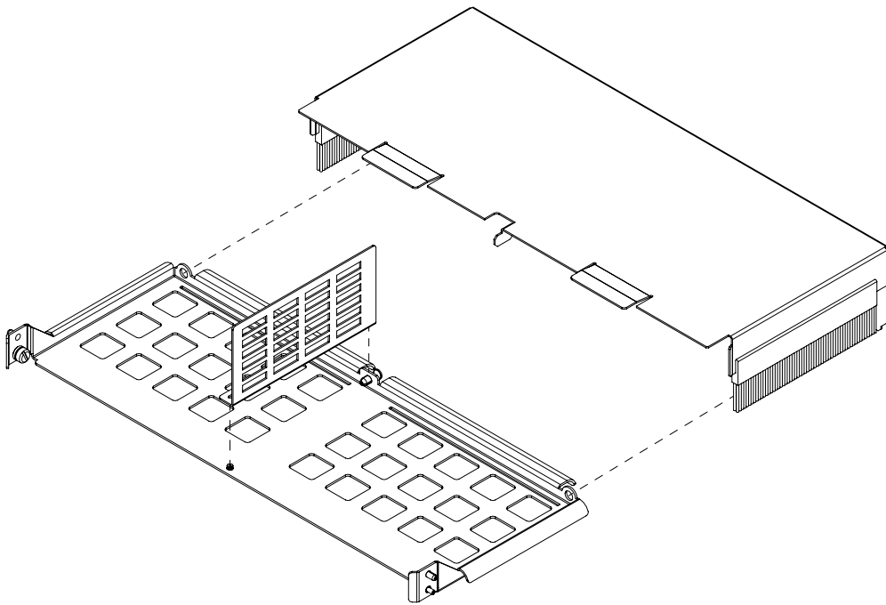
ISO VIEW
