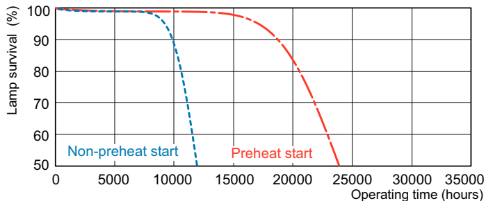
Life Expectancy Diagram - MASTER TL5 HE 14W/830 1SL/20
