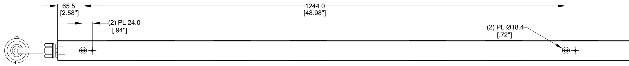
REAR VIEW
