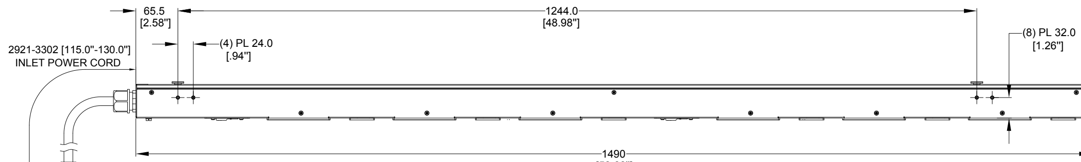
TOP VIEW
