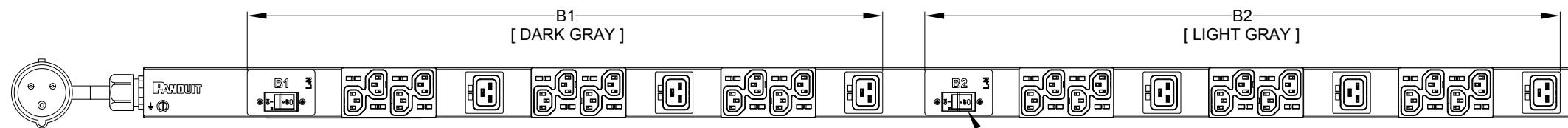
FRONT VIEW
