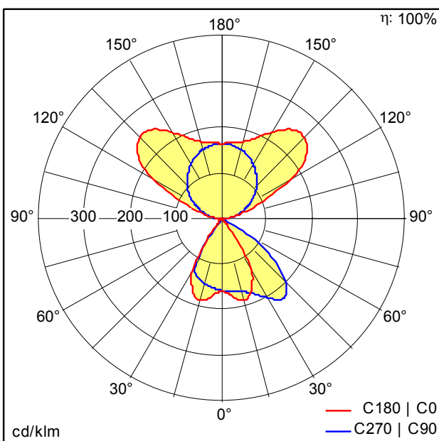
D37028AA_D37029AA_LINETIK-S_DI_LED8000-830_BK.Idt
