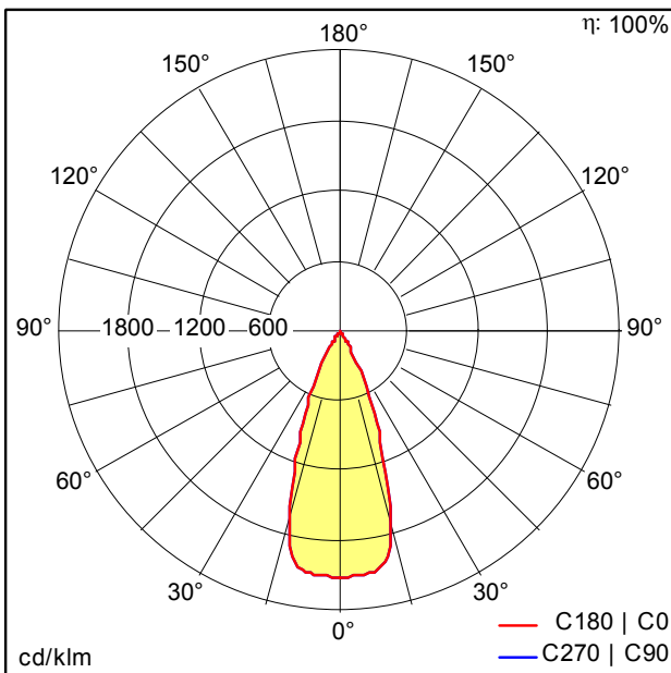
SUSY_S_1P_LED140-830_WFL.Idt, SUSY_S_1P_LED140-830_WFL.Idt, SUSY_S_1P_LED140-830_WFL.Idt
