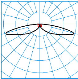
CS 19 100-SB3L/1200-730 2G1S ETDD (CLO initial value) TX300144 ■ C0 - C180 ■ C90 - C270 DIN 5040: A20 UTE: 1,00 J CEN Flux Code: 22 52 84 100 100 0 0 0 0
