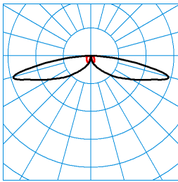
CS 19 100-SB3L/1200-730 2G1S ETDD (CLO end value) TX300143 ■ C0 - C180 ■ C90 - C270 DIN 5040: A20 UTE: 1,00 J CEN Flux Code: 22 52 84 100 100 0 0 0 0
