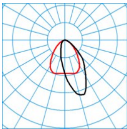
ELINE LAN40-110 ML 865 L150 2 50 ■ C0 - C180 DIN 5040 2 = A50 UTE 2 = 0.98 C + 0.02 T CEN flux code = 63 89 98 98 100 0 6 44 2
