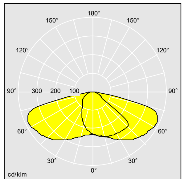
TL_CTL36L70NR730.ltd
