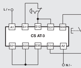
Input configuration with manual start 1 channel
