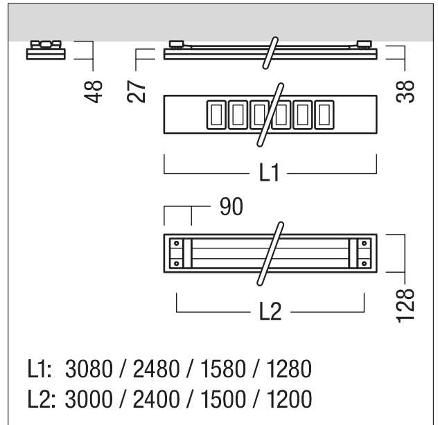
ZS_CEV_M_CLARIS_Evo_Surface_Mounted.wmf
