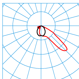
Jovie 50I-AM2L-LRA/3200-730 4G1 ET (CLO initial value) TX301467 ■ C0 - C180 ■ C90 - C270 DIN 5040: A40 UTE: 1,00 F CEN Flux Code: 47 91 100 100 100
