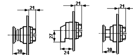
Schlagtaster "NOT-AUS" Schalter Schlagtaster "Mushroom-head EMERGENCY STOP" Potentiometer "Mushroom-head EMERGENCY STOP"
