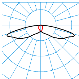
LIQ 50N-SB3L-LR/1800-740 2G1 ET (CLO end value) TX277687 ■ C0 - C180 ■ C90 - C270 DIN 5040: A30 UTE: 1,00 l CEN Flux Code: 31 64 92 100 100
