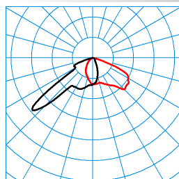
LIQ 70N-FL1L/6800-730 8G1 ET(CLO end value) TX277772 ■ C0 - C180 ■ C90 - C270 DIN 5040: A40 UTE: 1,00 F CEN Flux Code: 43 84 100 100 100
