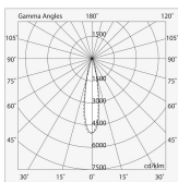
Fascio/Beam: 15°
