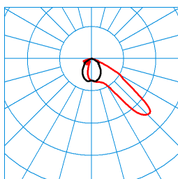
Jovie 50I-AM2L-SLR3/4200-740 4G1 ET (CLO initial value) TX300954 ■ C0 - C180 ■ C90 - C270 DIN 5040: A40 UTE: 1,00 F CEN Flux Code: 47 91 100 100 100
