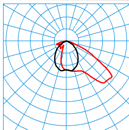
LnStar 40-AM2L-SLR3/10000-740 12G1S TX122216 ■ C0 - C180 ■ C90 - C270 DIN 5040: A40 UTE: 1,00 D CEN Flux Code: 48 88 99 100 100
