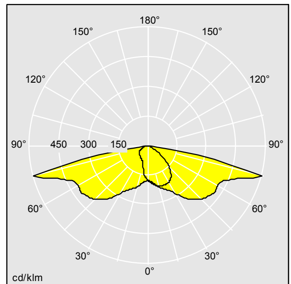
TL_CQS12L35WS740.ltd
