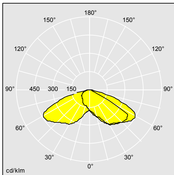
TL_EP36L70SC730.ltd
