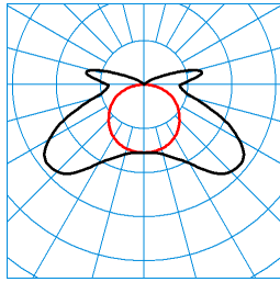
Aragon F 12 P-XW 3200/16ML-840 PC -4 TX113462
