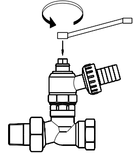
DANFOSS RLV-012-1
