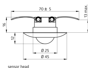
sensor head
