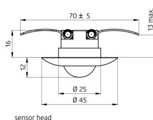
sensor head
