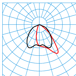
Jovie 70I-AM3L-LRA/6800-740 8G1 ET (CLO end value) TX301795 ■ C0 - C180 ■ C90 - C270 DIN 5040: A50 UTE: 1,00 D CEN Flux Code: 59 89 100 100 100
