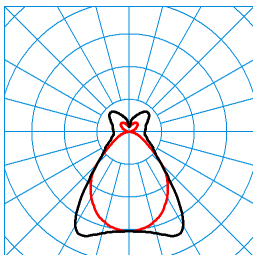
E-Line 7651 HE PMW19 40-830ET L150 01 TX375025 ■ C0 - C180 ■ C90 - C270 DIN 5040: B42 UTE: 0,72 D + 0,28 T CEN Flux Code: 60 83 93 72 100 26 59 82 28
