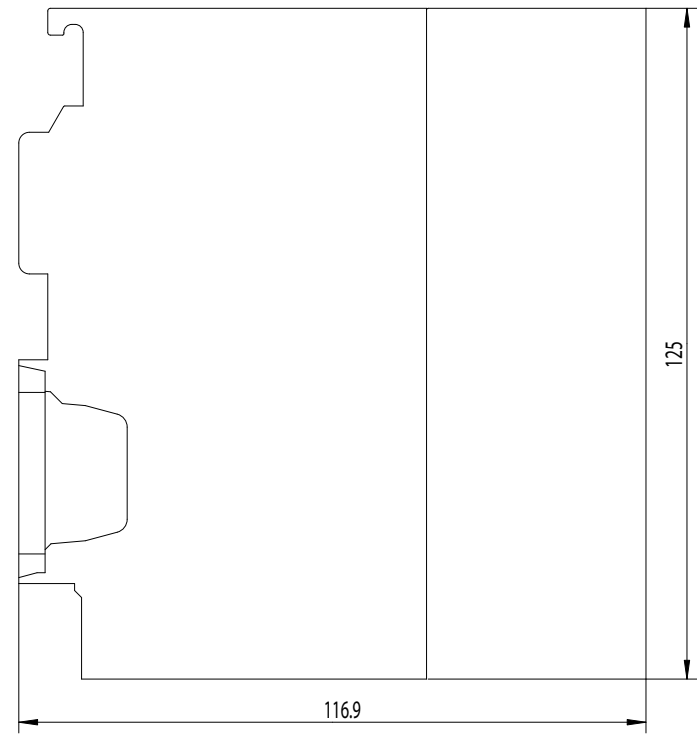
Links / Left
