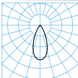
Faciella 15 RB2L/800-red 1G1 TX045298 ■ C0 - C180 DIN 5040: A70 UTE: 1,00 A CEN Flux Code: 90 98 100 100 100
