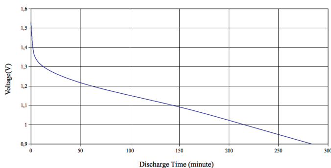
3.9Ω Continuous Discharge Curve
