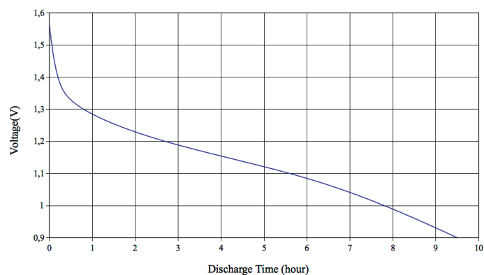
6.8Ω 1hour/day Discharge Curve
