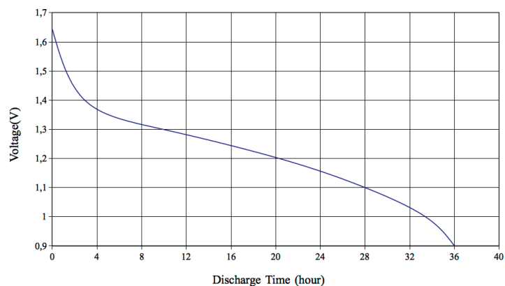
20Ω 4hour/day Discharge Curve
