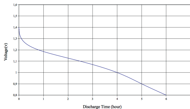
3.9Ω 1hour/day Discharge Curve
