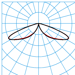
LTX PT-RB6L-LRA/15/18/26-740 4G1 (1800 lm) TX084174 ■ C0 - C180 ■ C90 - C270 DIN 5040: A20 UTE: 1,00 J CEN Flux Code: 15 51 96 100 100 0 0 0 0
