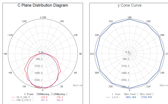
Lighting Distribution Diagram
