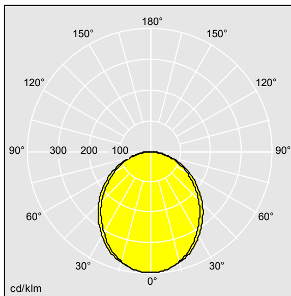
D44260AA_EQL_840_HF_L1000_PM_WH_.ldt
