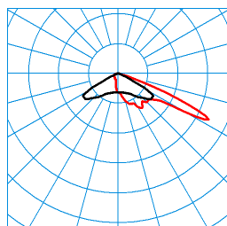
LnPlus 60-AM19L-LR/24000-730 18G1 ET (CLO initial value) TX376915 DIN 5040: A30 UTE: 1,00 J CEN Flux Code: 28 76 99 100 100
