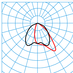
Jovie 70I-AM3L-SLR1/10000-730 8G1 ET TX195561 ■ C0 - C180 ■ C90 - C270 DIN 5040: A50 UTE: 1,00 D CEN Flux Code: 59 89 100 100 100
