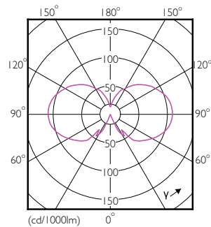
LEDBulb CLA 11-100W E27 A70 Clear 827 ND
