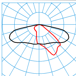
LIQ 50-AB2L-LRA/1350-730 2G1S TX054111 ■ C0 - C180 ■ C90 - C270 DIN 5040: A30 UTE: 1,00 G CEN Flux Code: 36 71 96 100 100
