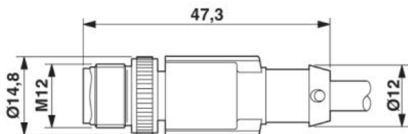
Dimensioned drawing, M12 plug
